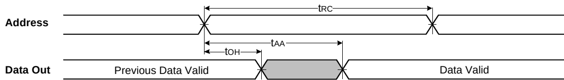
TIMING WAVEFORM OF READ CYCLE(1) (Address Controlled, \overline{\text{CS}}=\overline{\text{OE}}=\text{V}_{\text{IL}} , \overline{\text{WE}}=\text{V}_{\text{IH}} , \overline{\text{UB}} or/and \overline{\text{LB}}=\text{V}_{\text{IL}} )
